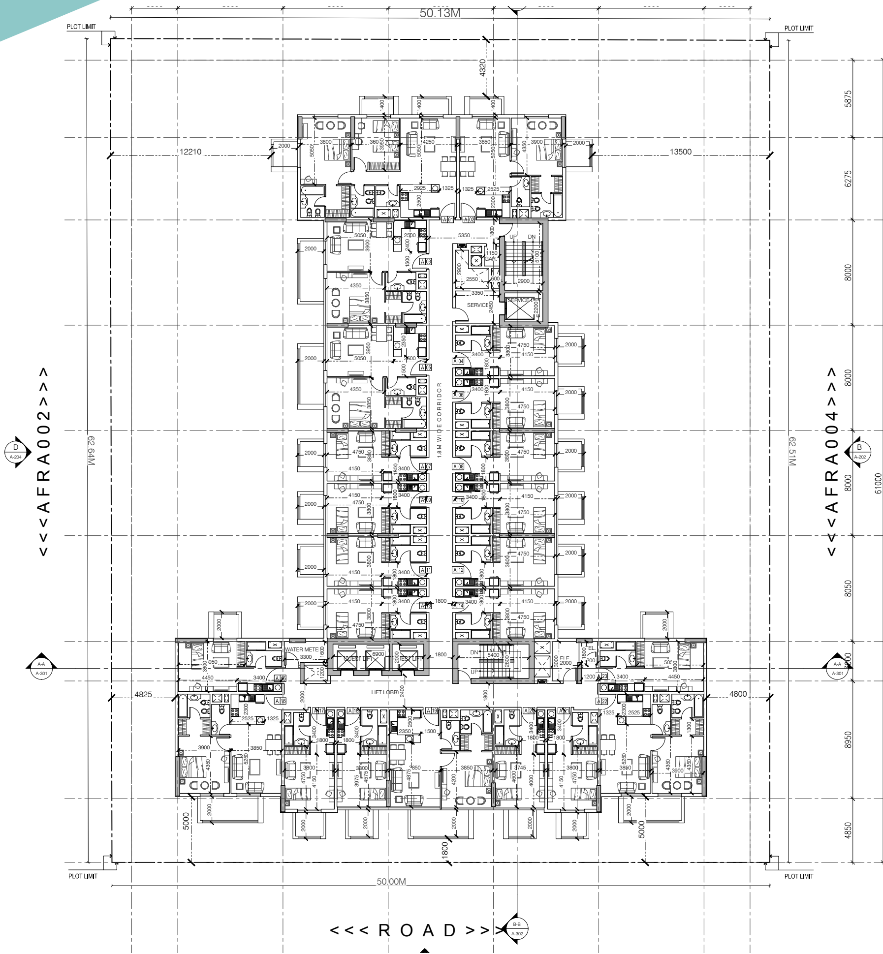
TYPICAL FLOOR
